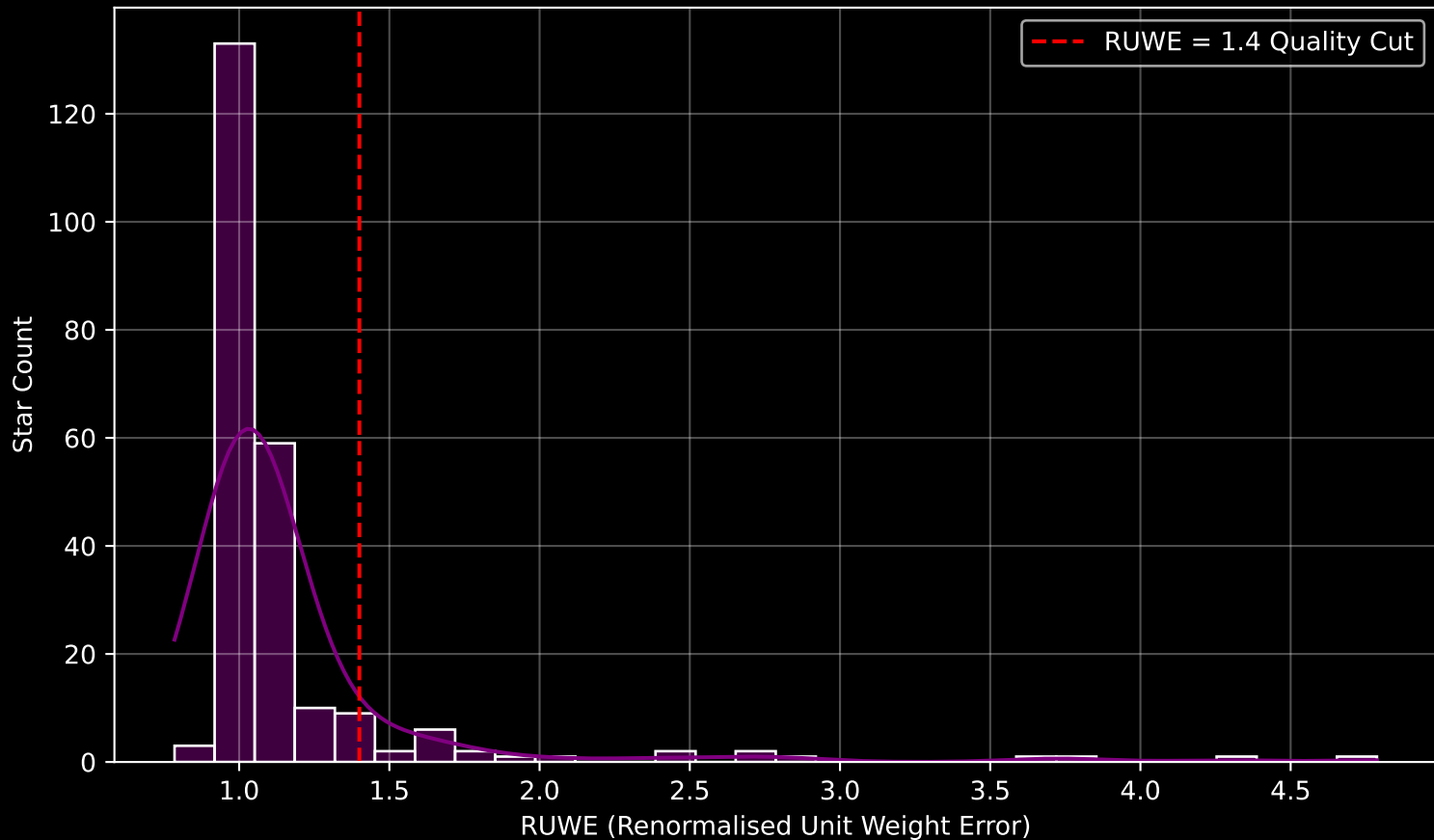
GALAH DR4 Field [6784] RUWE Distribution (n= 235)
