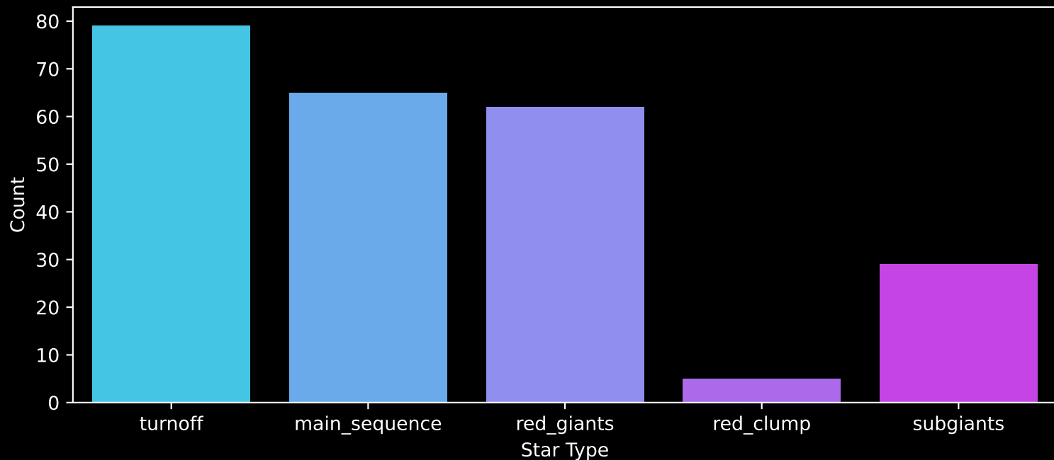
GALAH DR4 Field: [6784] Count plot of Star Type
