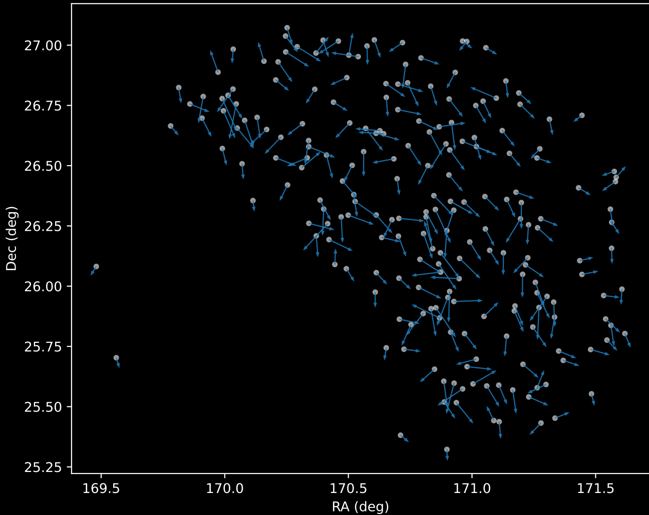
GALAH DR4 Cluster 0 Proper Motion Vectors (n=212)
